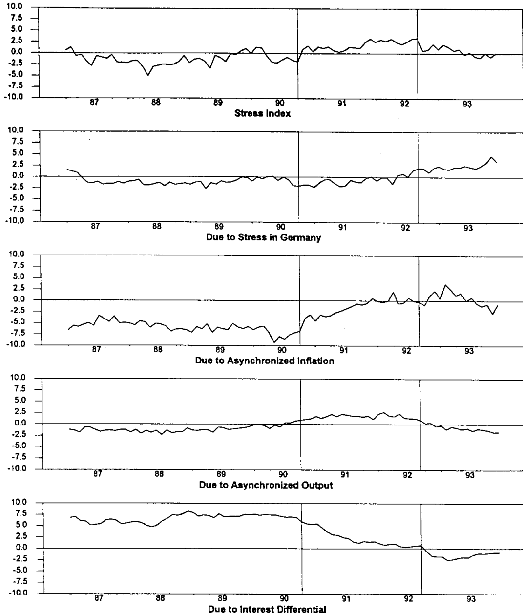
Figure 6: Stress in Britain
