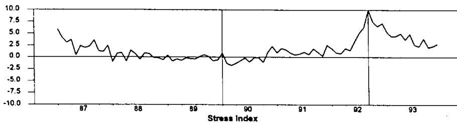
Figure 8: Stress in Italy
