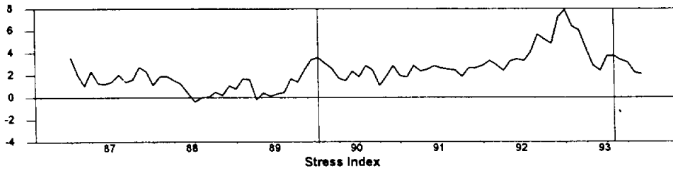
Figure 7: Stress in France
