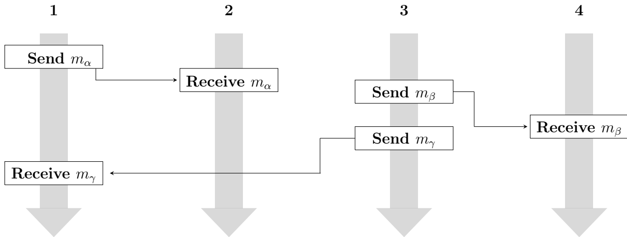
Figure 16: MPI computing
